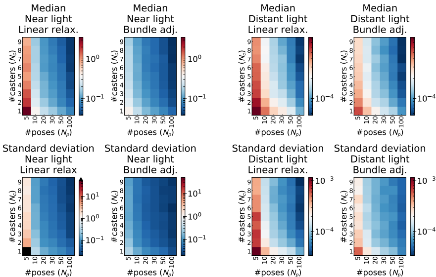
Fig. C.1. Estimation error for synthetic near and distant light with Gaussian noise added to shadow positions ( \sigma_{\text{shadows}} = 0.01 ) and board orientation in degrees ( \sigma_{\text{pose}} = 0.005 ). N_p is on the x-axis and N_c is on the y-axis. For each data point we performed 500 random trials. Top row: The median of the absolute error (near light)/angular error in degree (distant light). Bottom row: The error’s standard deviation.
