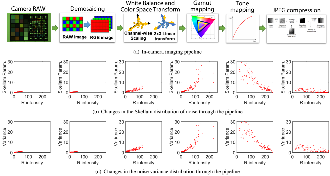
Figure 1. In-camera imaging pipeline and changes in noise distribution through the pipeline. (a) shows block diagram sequences of in-camera imaging pipeline. (b) and (c) show the changes in the Skellam and the variance distribution through the pipeline, respectively. Noise characteristic drastically changes with the gamut mapping and the tone mapping processes.
